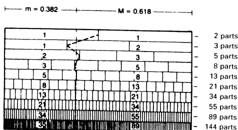
representation of the Lamesch Row from Neufert 'Bauproduktionslehre'
